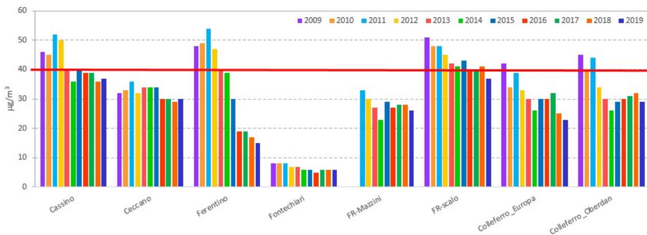
Figura 5.8 - Media Annua \text{NO}_2 .
